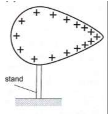
Charge distribution for an isolated pear-shaped conductor
